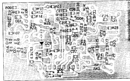
Solder side (reverse)
