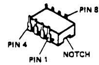
SN16913P (Q2009,2012)
