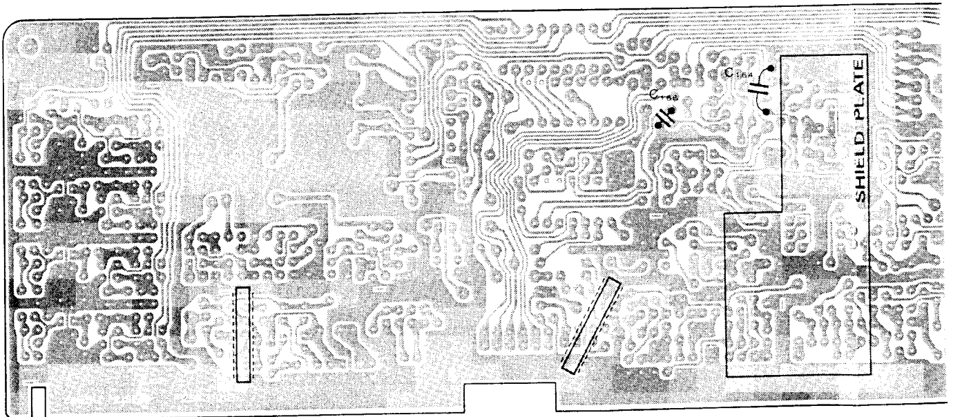
Solder side
