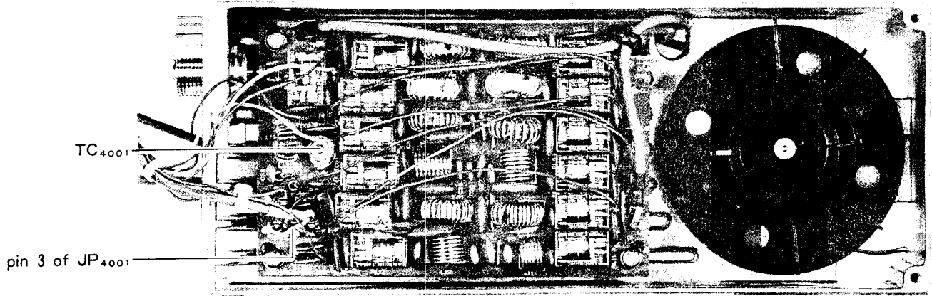
LPF UNIT ALIGNMENT POINTS
