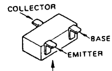
2SC3052F (Q8103,8104)
